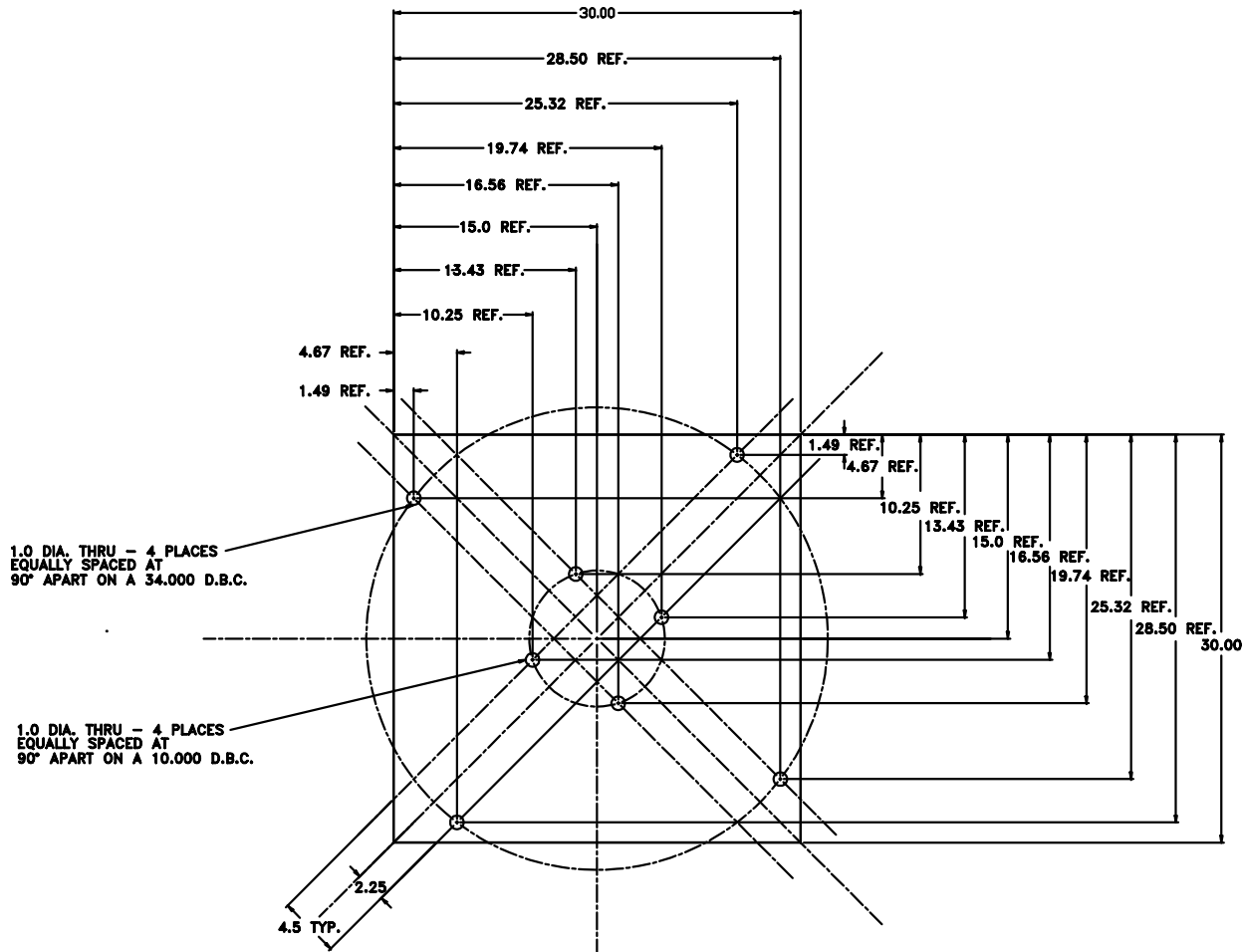
DETAIL - ITEM 2 [ .75 THK PLATE ]
